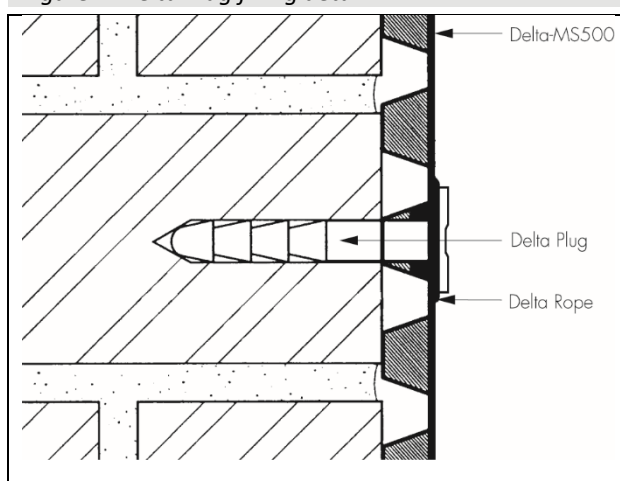
Figure 2 Delta Plug fixing detail
