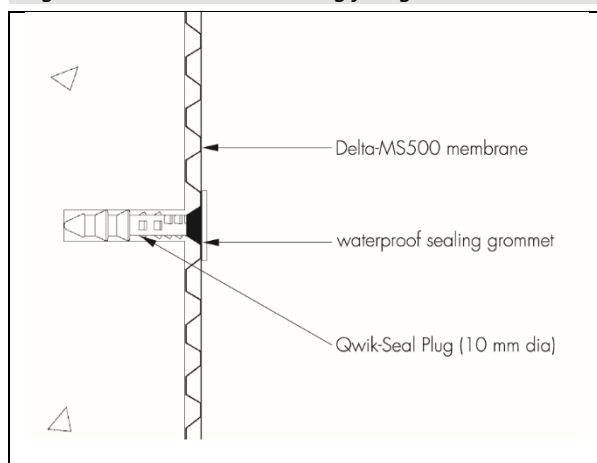
Figure 1 Delta Qwik-Seal Plug fixing detail
