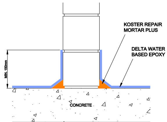
INTERNAL WALL / FLOOR DETAIL
