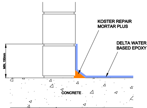
PARTY WALL / FLOOR DETAIL
