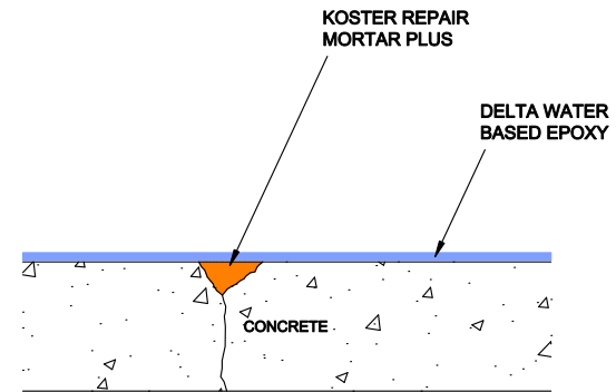
INTERNAL WALL / FLOOR DETAIL
