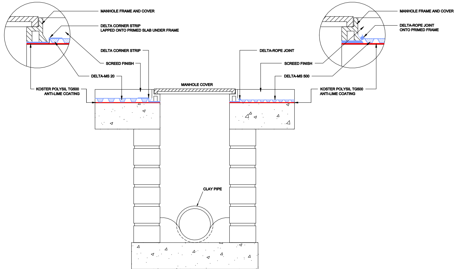
SEALING TO A MANHOLE
