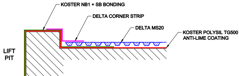
③ LIFT PIT / MS20 UPSTAND DETAIL
