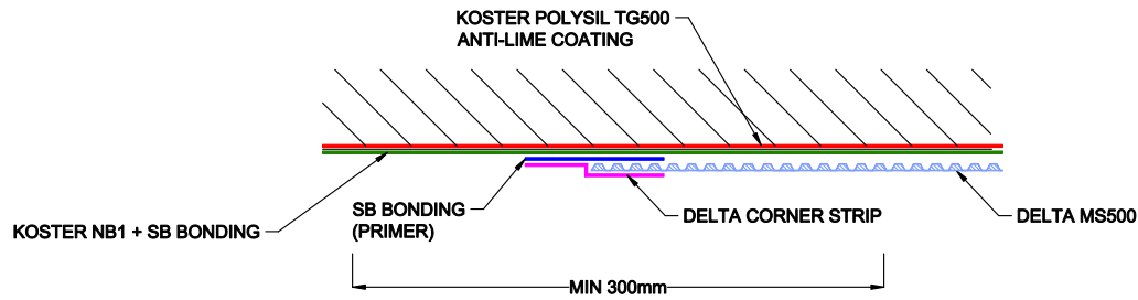
② NB1 / MS500 OVERLAP
