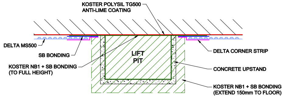
① LIFT PIT (PLAN VIEW)
