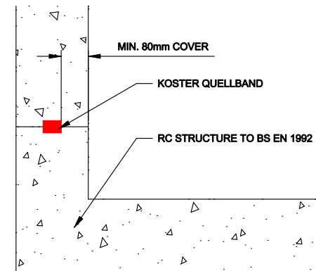
KICKER CONSTRUCTION
