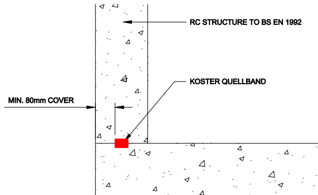
KICKERLESS CONSTRUCTION
