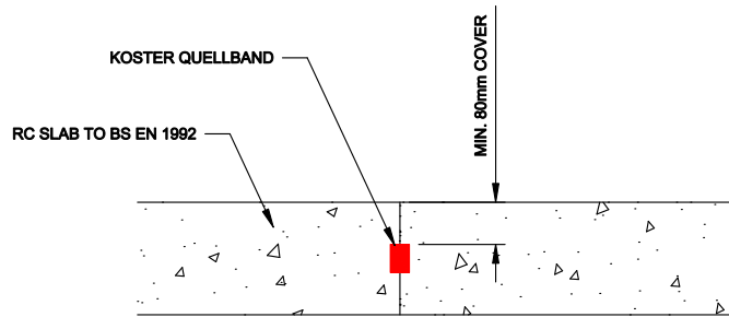
NEW SLAB CONSTRUCTION JOINT
