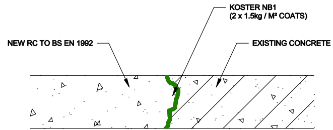
NEW TO EXISTING CONSTRUCTION JOINT
