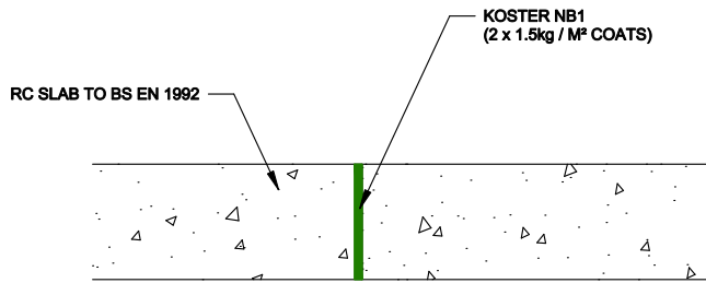
NEW SLAB CONSTRUCTION JOINT
