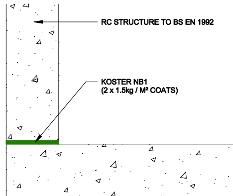
KICKERLESS CONSTRUCTION
