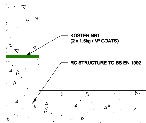
KICKER CONSTRUCTION
