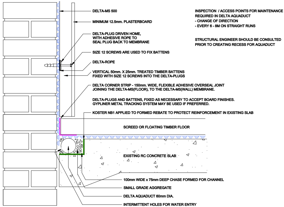
DELTA AQUADUCT SECTION
