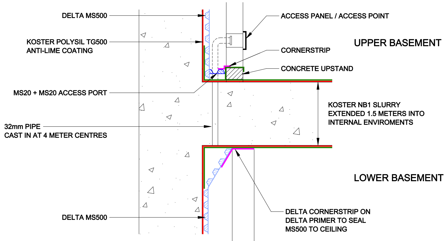
INTERMEDIATE SLAB DRAINAGE DETAIL
