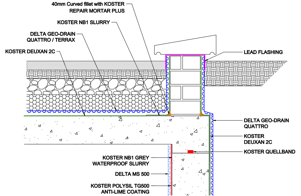
RC DECK DETAIL WITH BRICK WALL OFFSET TO RC WALL
