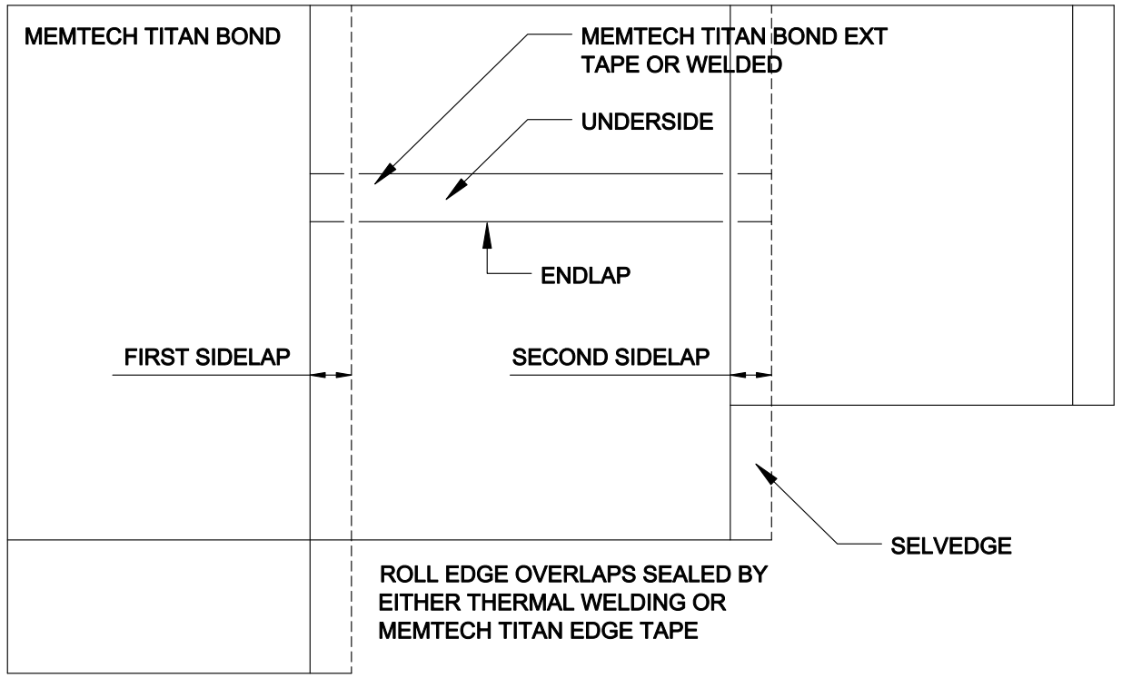
ROLL END OVERLAP DETAIL
