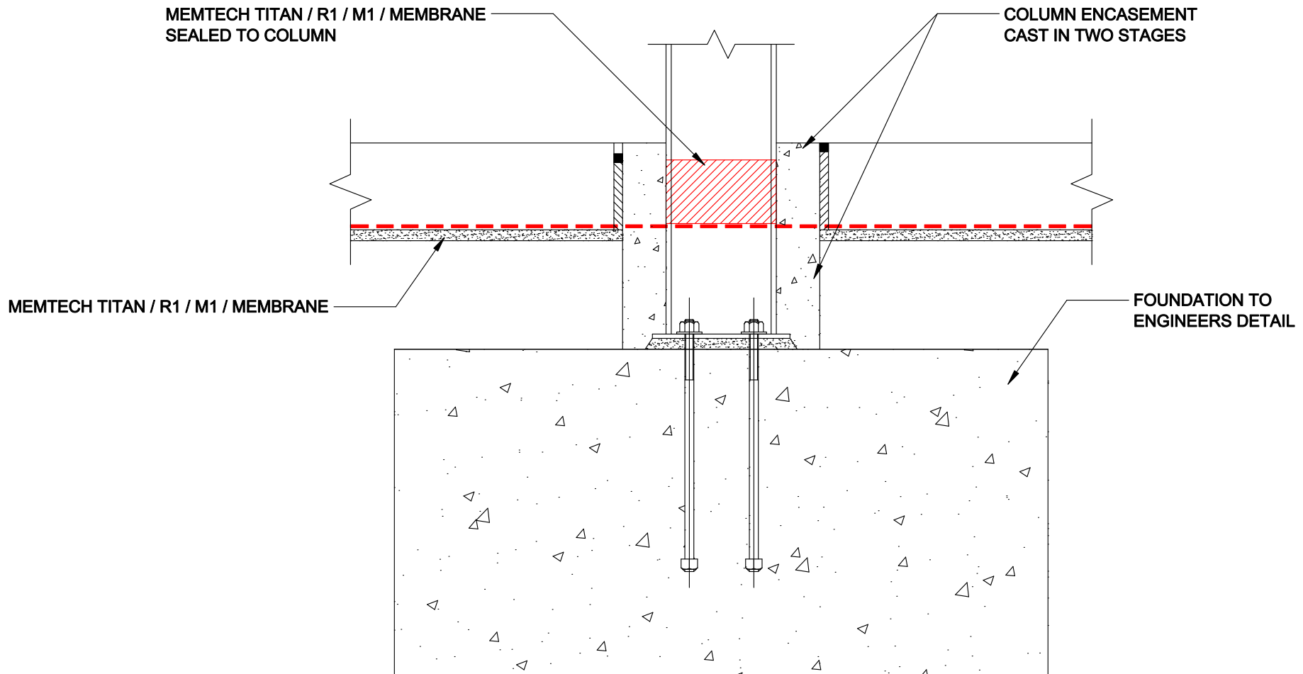
TYPICAL SLAB SECTION
