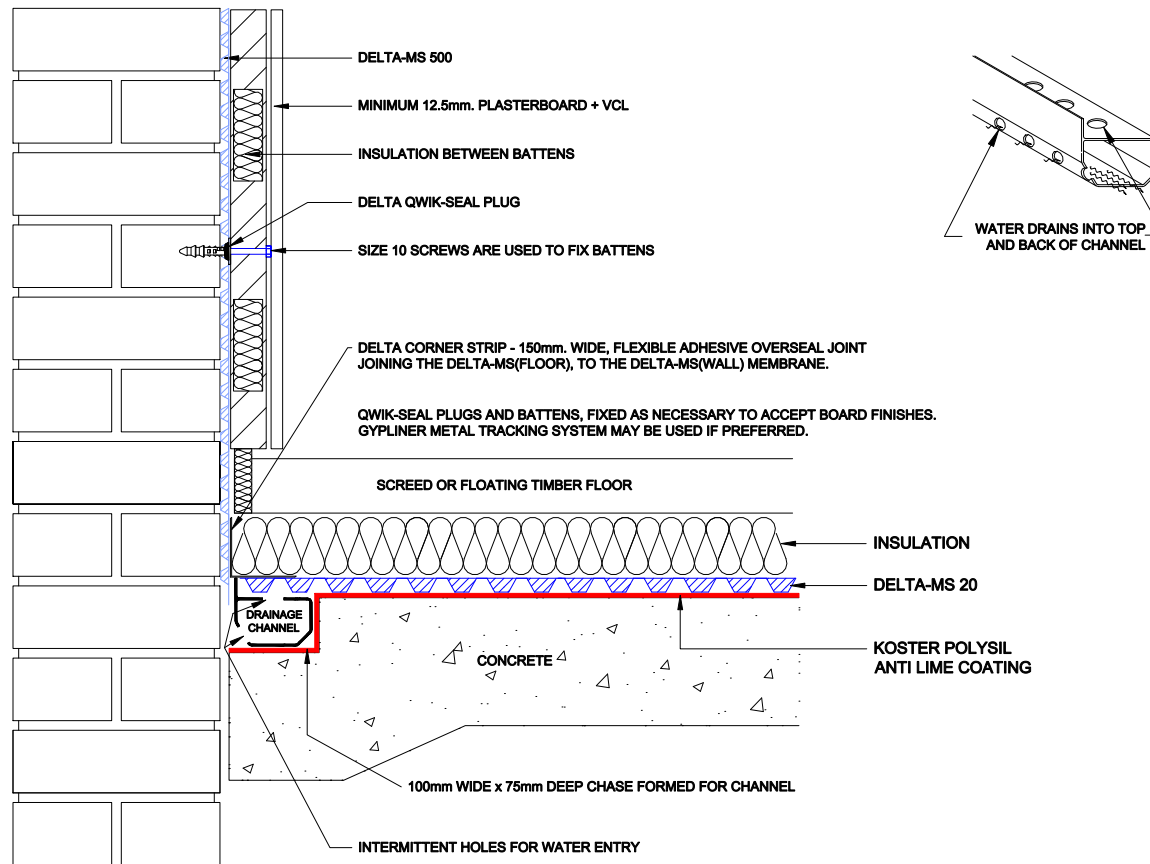
TYPE C, DRAINED PROTECTION, WALL AND FLOOR APPLICATION
