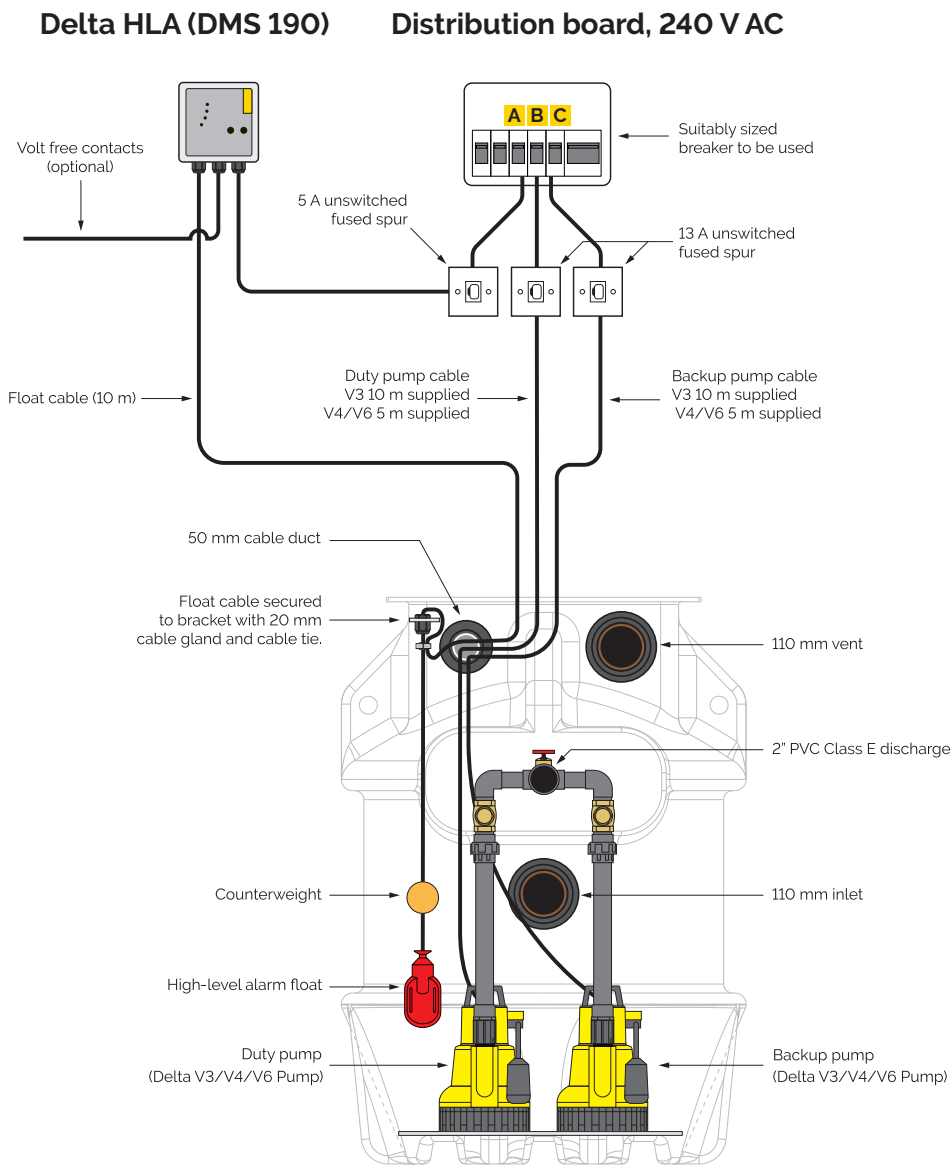
Delta 800 Dual V3/4/6 packaged pumping station
