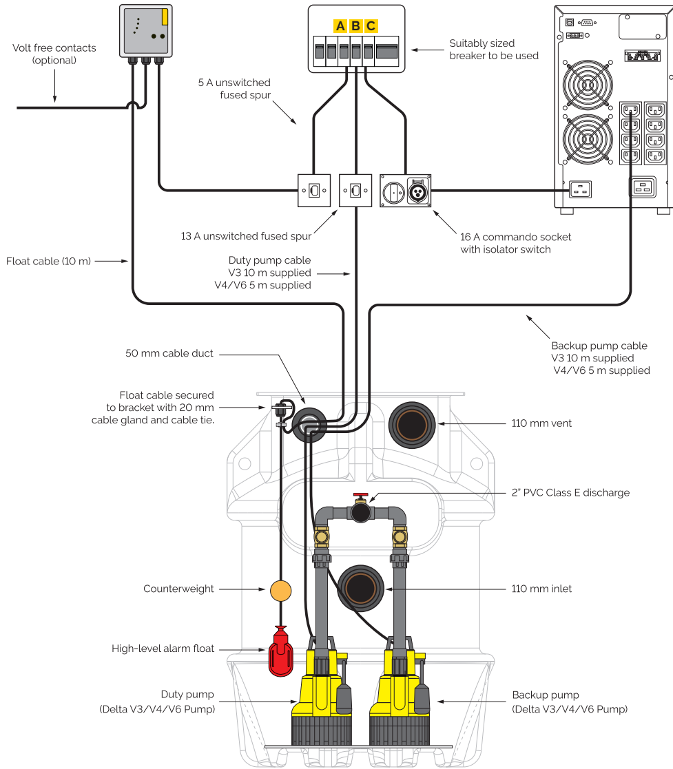
Delta 800 Dual V3/4/6 packaged pumping station
