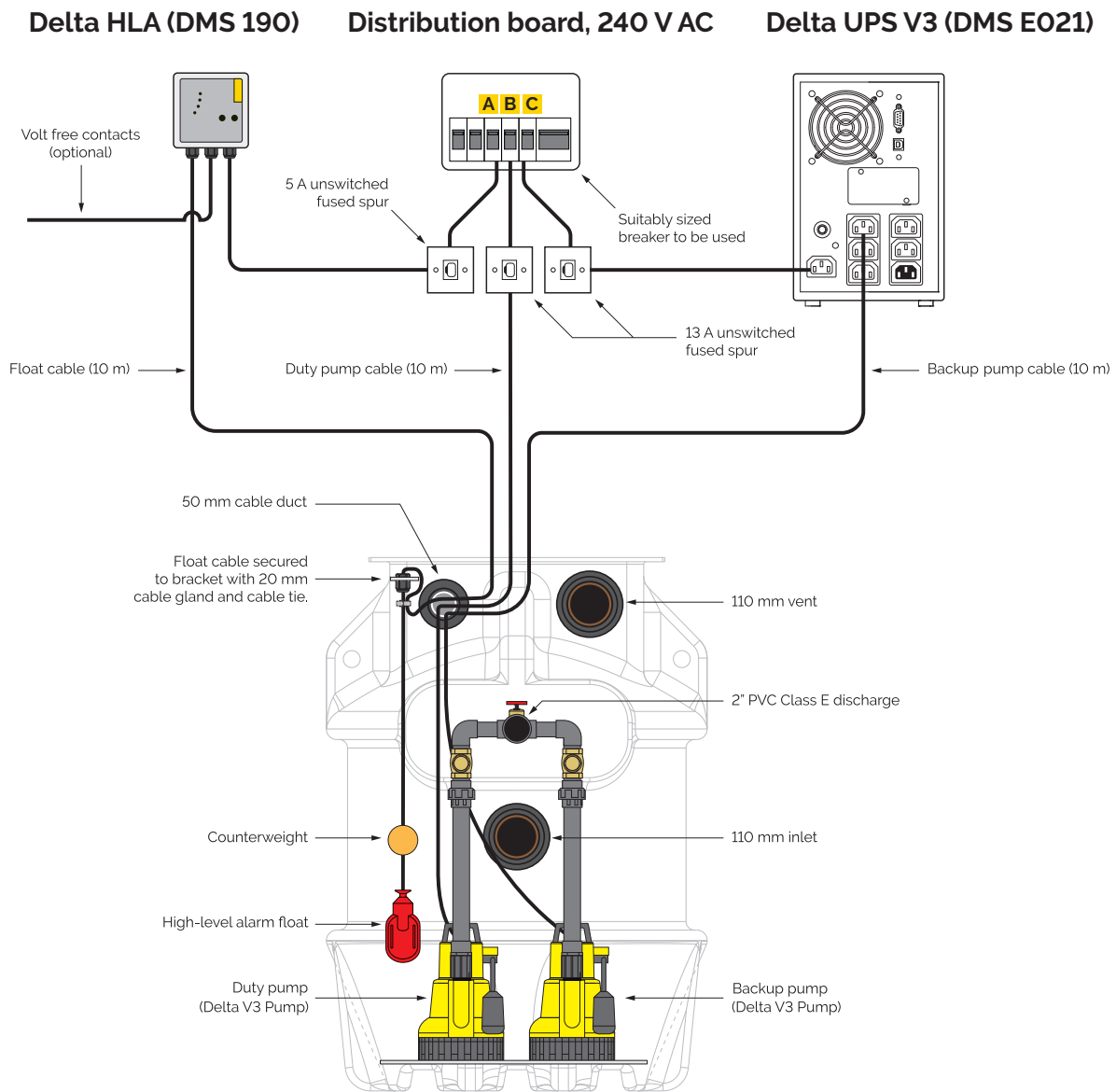
Delta 800 Dual V3 packaged pumping station
