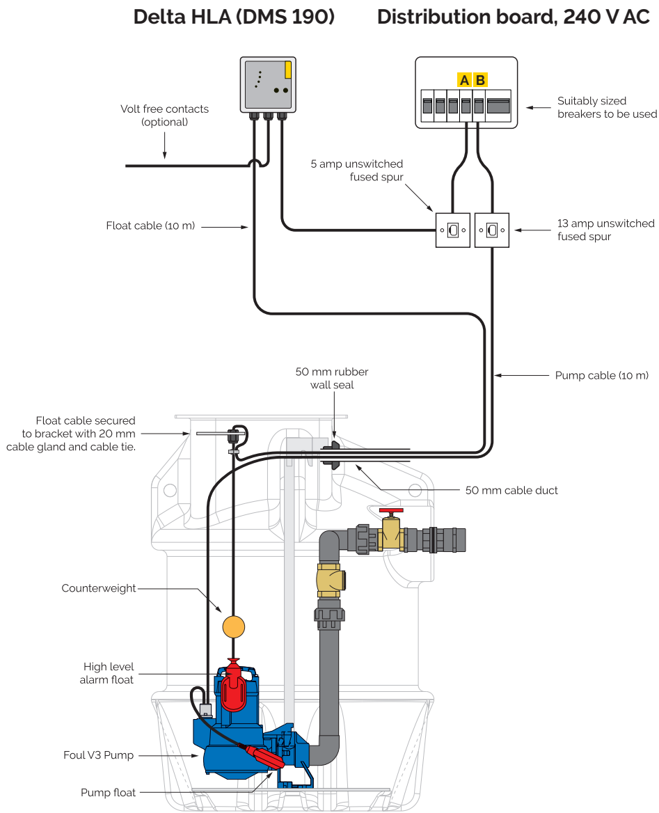
Delta 800 Single Foul V3 packaged pumping station
